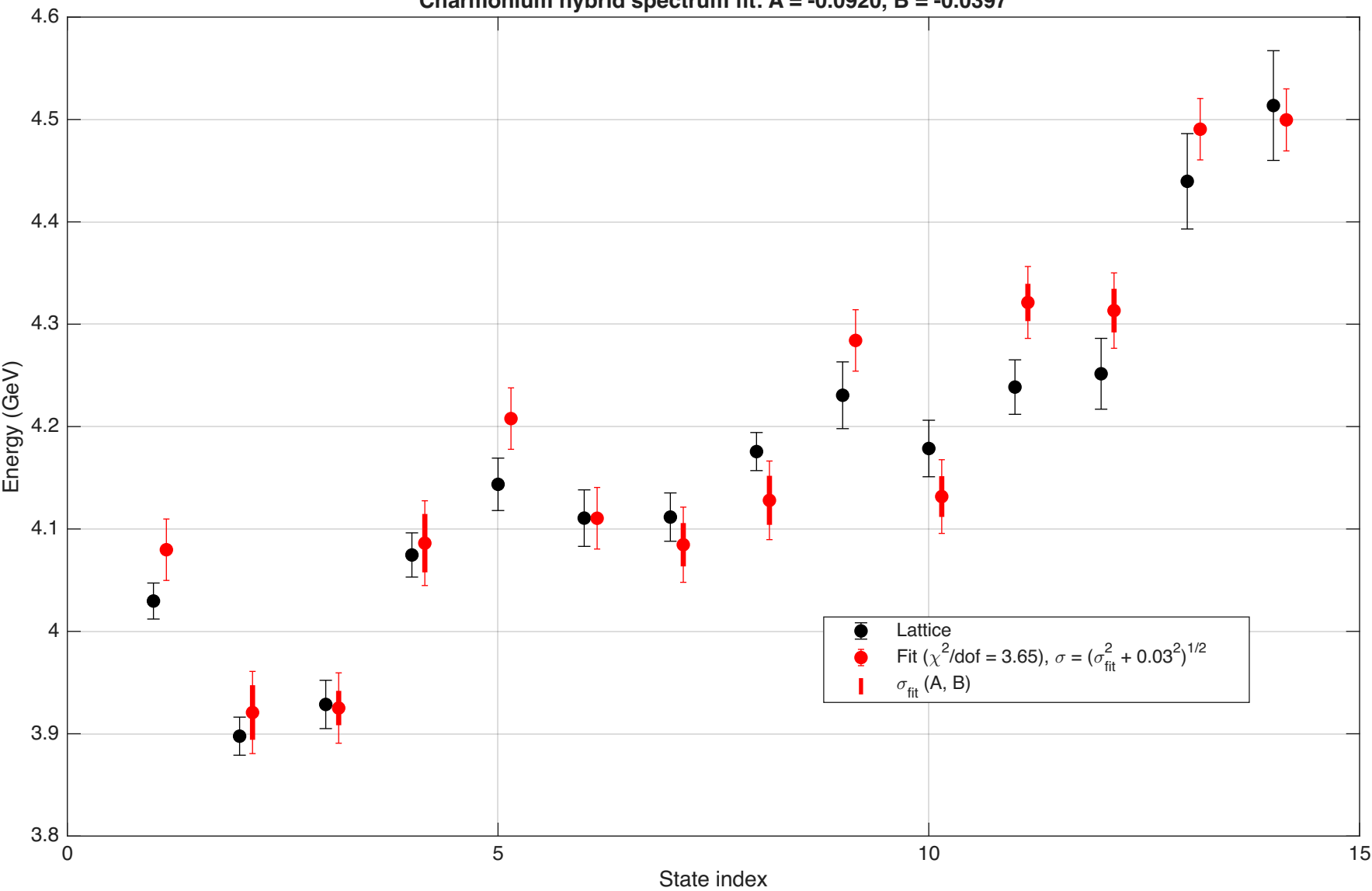
Charmonium hybrid spectrum fit: A = -0.0920, B = -0.0397
